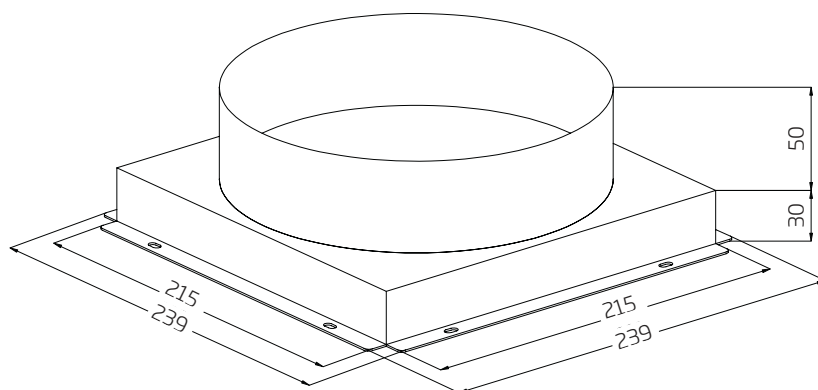
Dual 200mm adaptor
